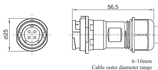
In-line cable connector C Mate with SY1710
