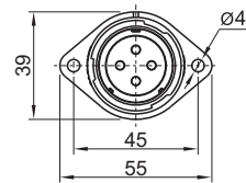
2-hole flange Mate with SY2910
